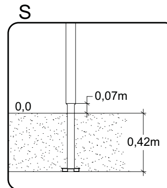
S Sunken Foundation 8112844
